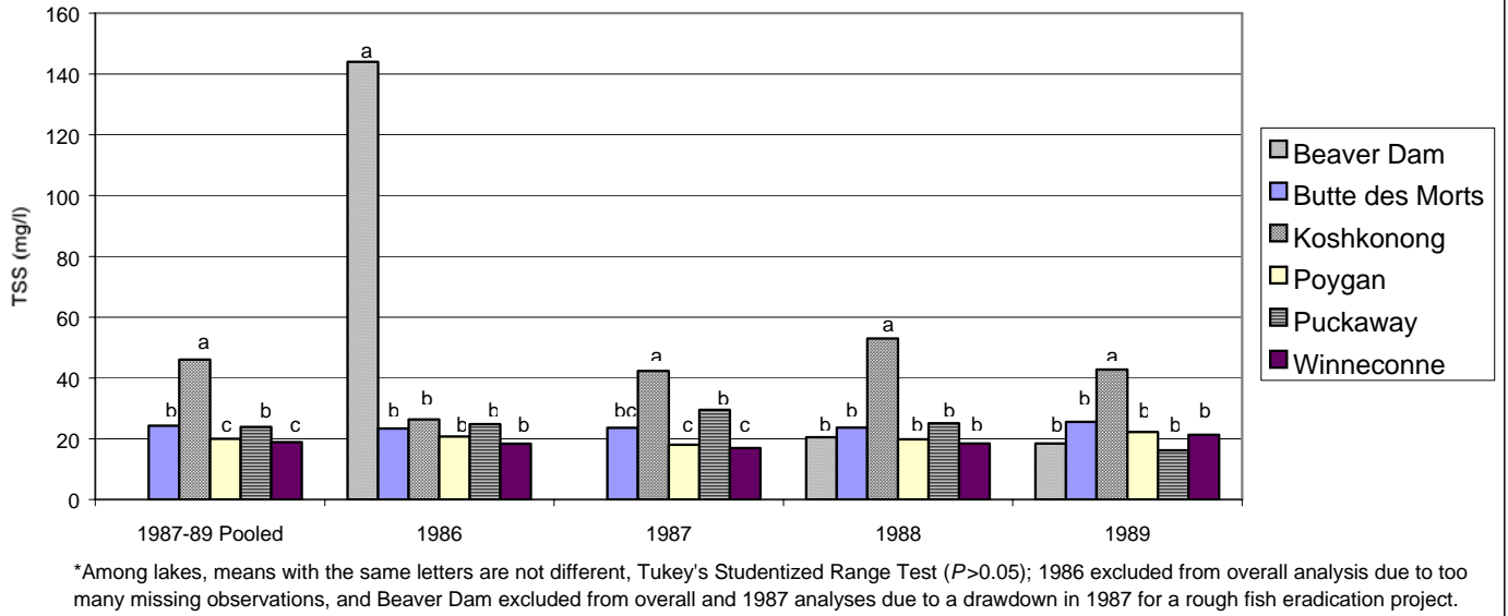
Figure 29 Mean total suspended solids (TSS) for 3 mid-lake sampling sites in each of 6 lakes in south and east central Wisconsin, late April-late August, 1986-89 (for 1987-89 pooled excluding Beaver Dam N=87-90; for 1986 N=22-27; for 1987 excluding Beaver Dam N=30; for 1988 N=30; for 1989 N=27-30).*
