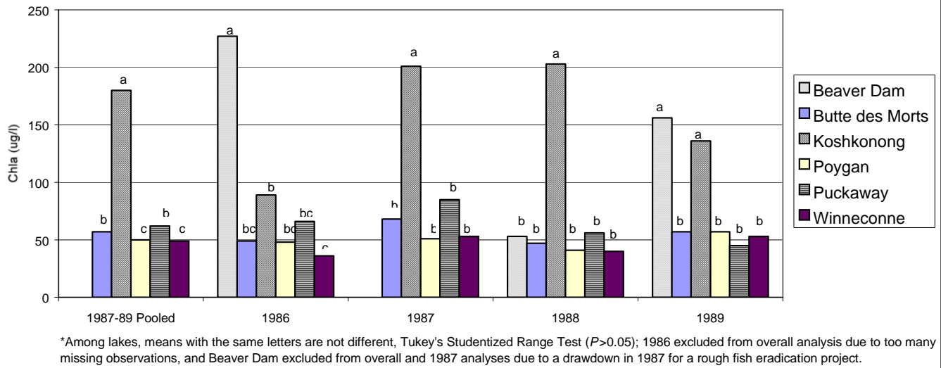
Figure 33 Mean chlorophyll a (chl a ) concentrations for 3 mid-lake sampling sites in each of 6 lakes in south and east central Wisconsin, late April-late August, 1986-89 (for 1987-89 pooled excluding Beaver Dam N=89-90; for 1986 N=22-27; for 1987 excluding Beaver Dam N=29-30; for 1988-89 N=30).*
