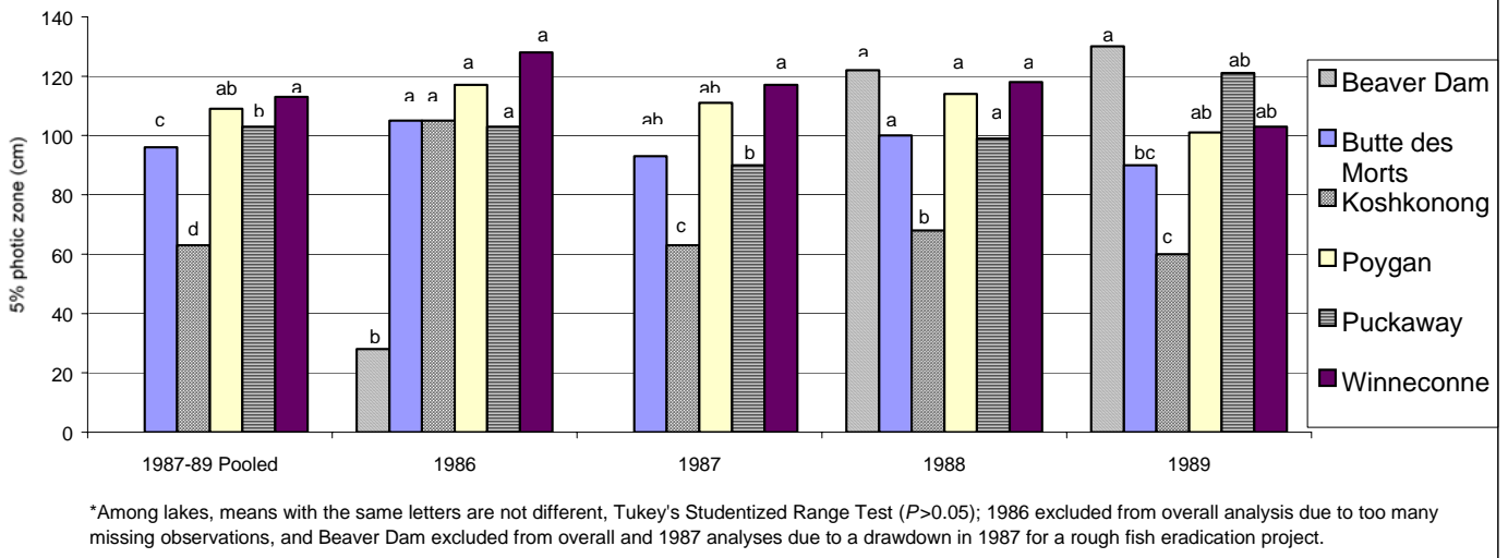
Figure 34 Mean 5% photic zone depth for 3 mid-lake sampling sites in each of 6 lakes in south and east central Wisconsin, late April-late August, 1986-89 (for 1987-89 pooled excluding Beaver Dam N=87-90; for 1986 N=22-25; for 1987 excluding Beaver Dam N=27-30; for 1988-89 N=30).*
