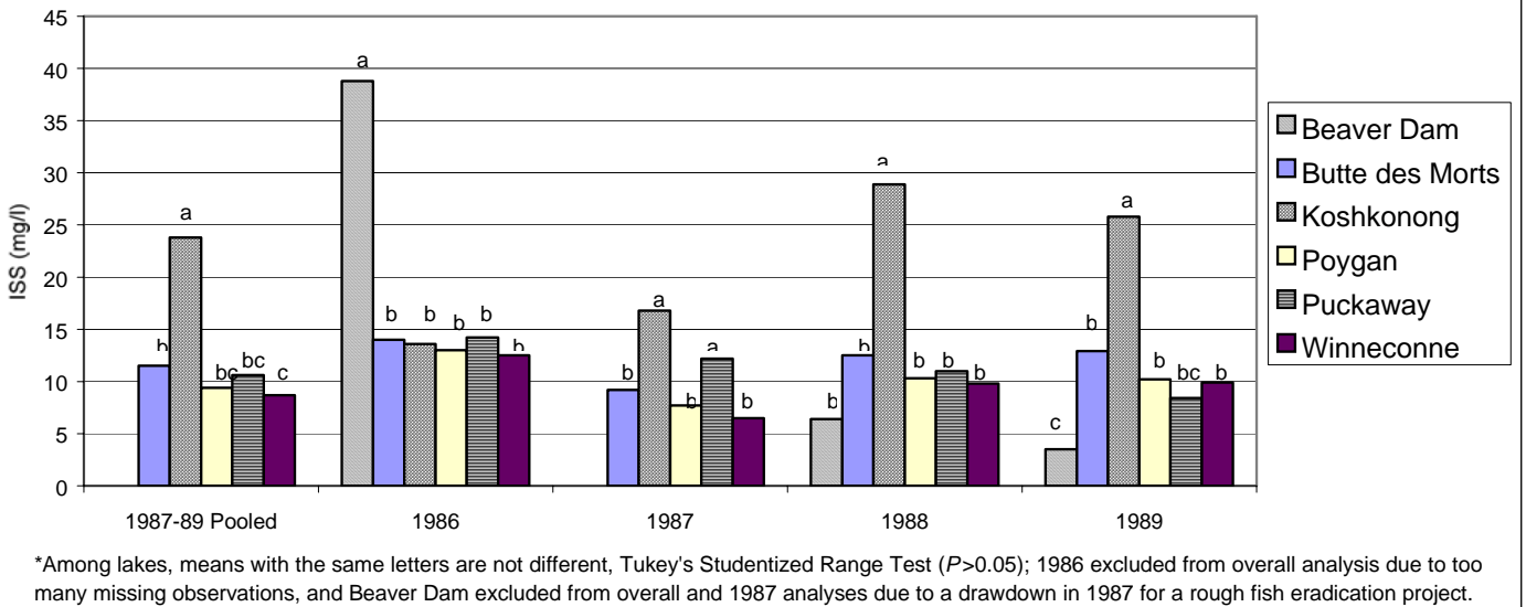
Figure 30 Mean inorganic suspended solids (ISS) for 3 mid-lake sampling sites in each of 6 lakes in south and east central Wisconsin, late April-late August, 1986-89 (for 1987-89 pooled excluding Beaver Dam N=87-90; for 1986 N=22-27; for 1987 excluding Beaver Dam N=30; for 1988 N=30; for 1989 N=27-30).*
