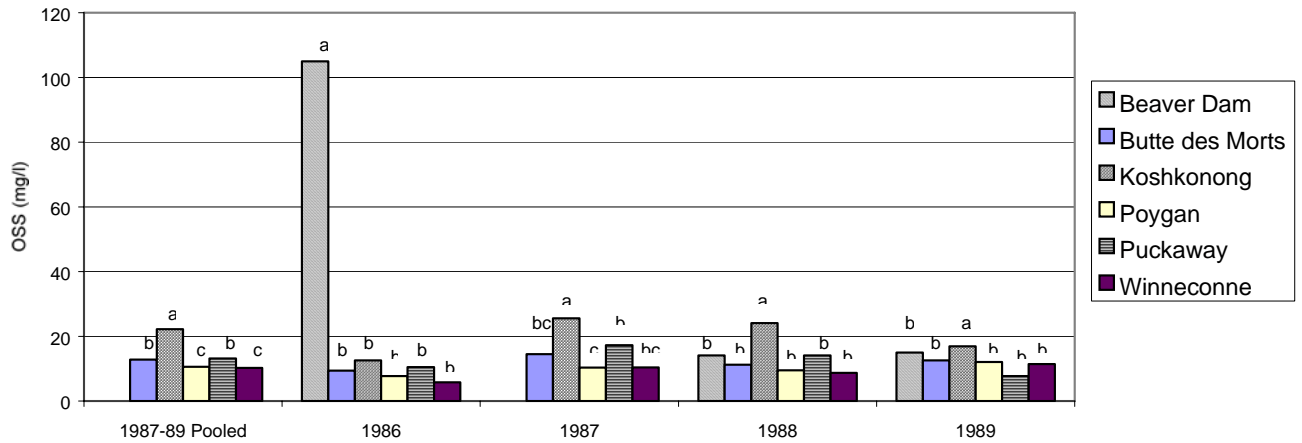
Figure 31. Mean organic suspended solids (OSS) for 3 mid-lake sampling sites in each of 6 lakes in south and east central Wisconsin, late April-late August, 1986-89 (for 1987-89 pooled excluding Beaver Dam N=87-90; for 1986 N=22-27; for 1987 excluding Beaver Dam N=30; for 1988 N=30; for 1989 N=27-30).*
